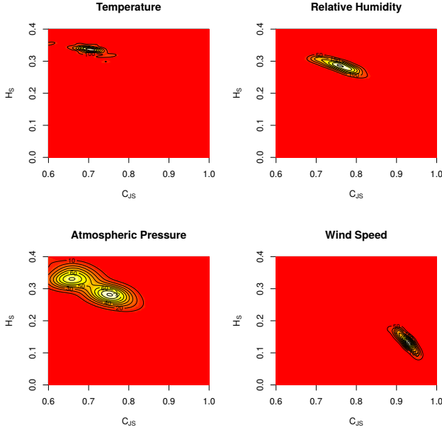
Fig. 7. Heat map illustrating the concentration of points from information quantifiers related to the characterization of the temperature, relative humidity, atmospheric pressure, and wind speed phenomena, with D = 6 .
