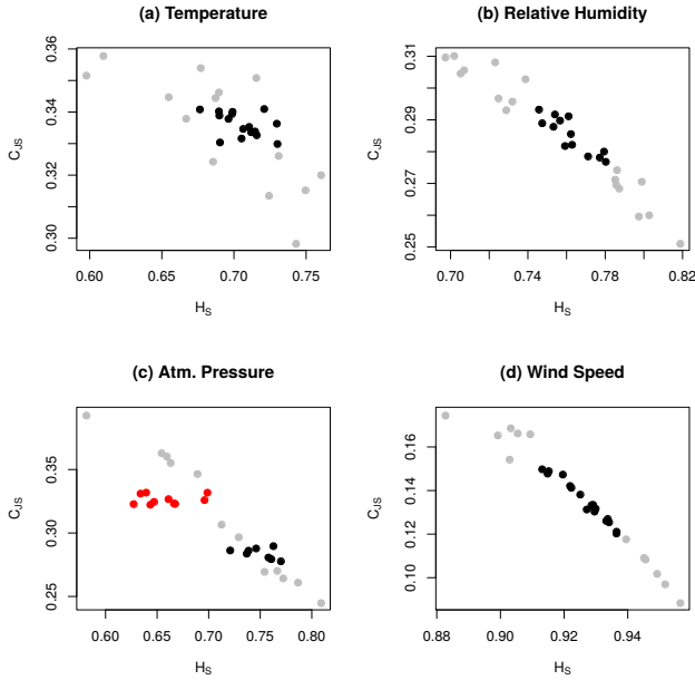
Fig. 8. Most relevant points discovered by Skinny-dip clustering algorithm for the physical phenomena, with D = 6 .
