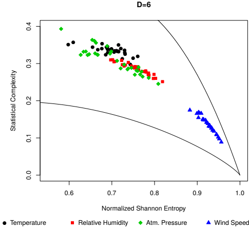
Fig. 5. CCEP of historical weather data in the period between years 2000 and 2015 of all the places used for characterization, with D = 6 .
