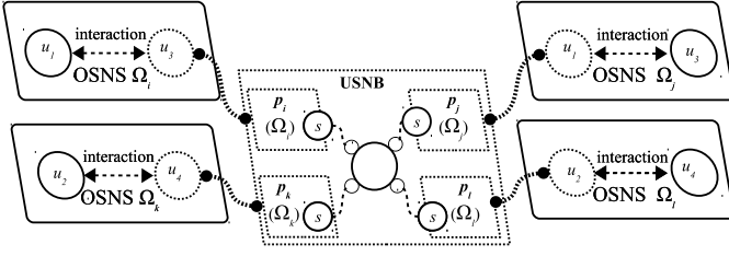
Fig. 3: The USNB multi-party distributed mediation across online social network services.
