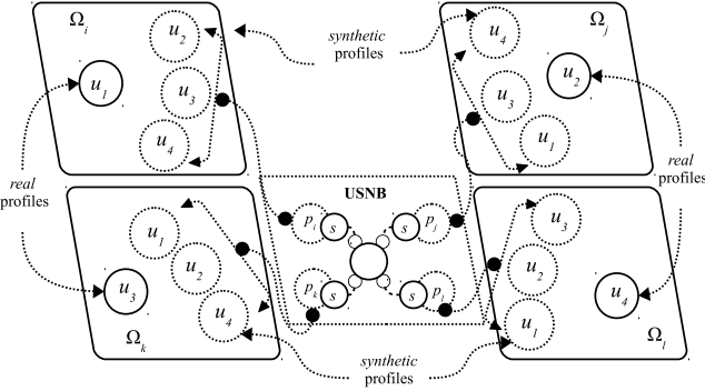
Fig. 4: Federating heterogeneous OSNs via USNB and synthetic profiles (depicted using dotted circles).
