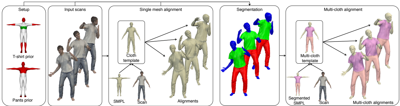
Fig. 2. Outline. Three main steps are needed to obtain multi-cloth alignments: single mesh alignment, scan segmentation and multi-cloth alignment. Multi-cloth alignment garments can be easily retargeted to novel shapes.
