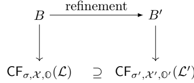
Figure 3: Anti-monotony of the counterfactual builder under refinement of the behavioral model.
