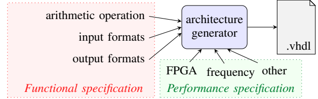
Fig. 1. The interface to an arithmetic generator
