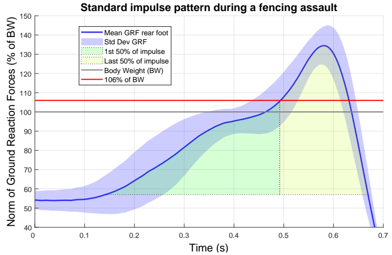
Figure 2. The ground reaction force threshold triggering the target motions was set so that half of the total impulse of a standard fencing assault had been produced. The mean ground reaction force norm leading to this condition corresponded to 106% of the subject body weight.
