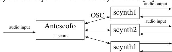
Figure 4. Antescofo launches several scsynth servers, for instance, one per core on the processor. It watches the load on the server and tries to place new synths on the least loaded servers.
