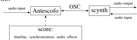
Figure 2. AntesCollider does not use the sclang client for audio routing and interacts directly with the scsynth audio server. The Antescofo score describes the timeline, the synchronization strategies and the audio effects, and scsynth processes the audio.
