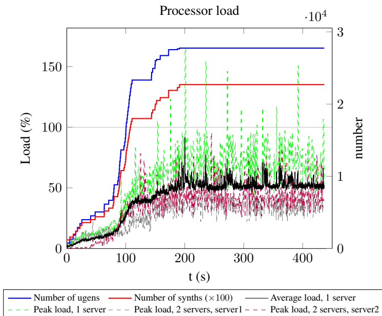
Figure 5. The CPU load (calculated as a moving average), peak CPU load, number of unit generators and number of synths, during an execution of the piece Curvatura II on one server. We also show the peak load on each server for the execution of the same piece with the same timings, load-balanced on two servers. A synth is made of several ugens. We scaled the number of synths by 100 on the graph, to make it visible.
