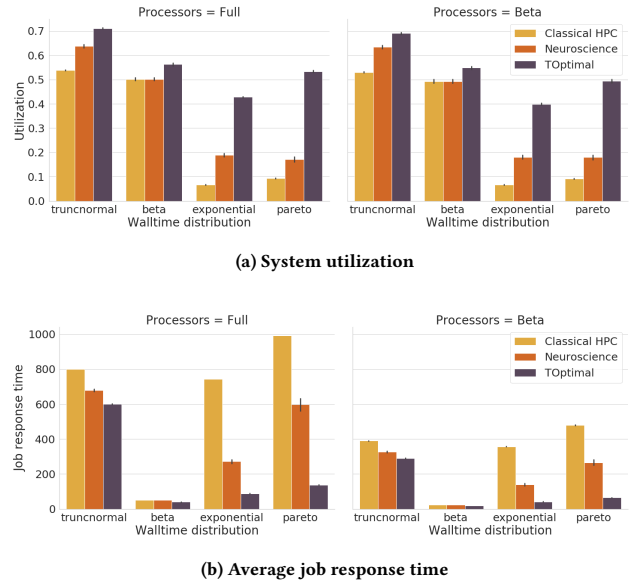
Figure 2: System utilization and average job response time under different walltime distributions for jobs that occupy the entire machine (Full) and jobs whose processor allocations follow the Beta distribution.
