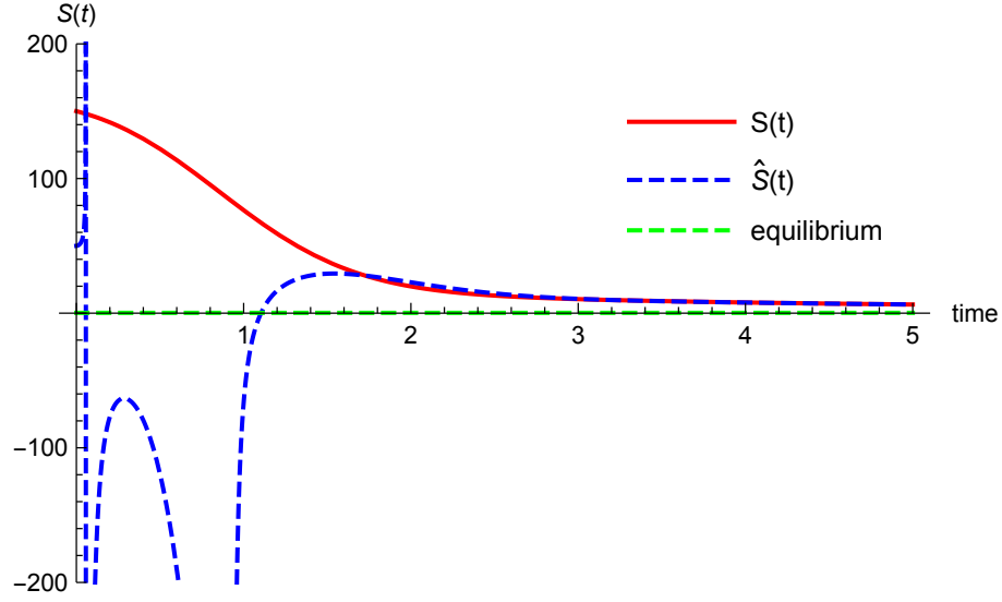
Figure 5: The evolution of S(t) and its estimate \hat{S}(t) delivered by the high-gain observer (11). One can notice a very important initial overshoot (for t < 1 ) of the estimate.
