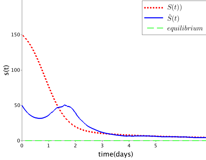
Figure 2: The evolution of S(t) and its estimate \hat{S}(t) delivered by the observer (13) when the measurable output is corrupted by noise.
