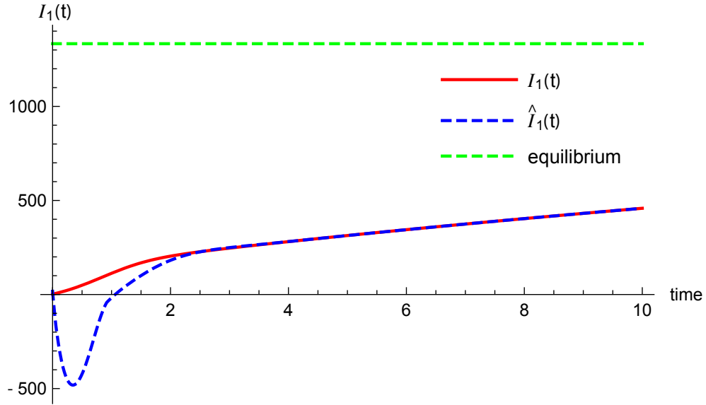
Figure 6: The evolution of I_1(t) and its estimate \hat{I}_1(t) delivered by the high-gain observer (11). Once again there is an initial overshoot of the estimate.
