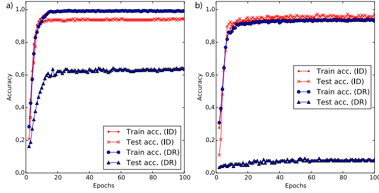
Fig. 2. Training- and test-set accuracy over 100 epochs for the best performing dataset A (a) and the worst performing dataset F (b) with a FFNN (1 hidden layer, 50 neurons). Despite around 3000 samples, our dataset is comparably small and the networks converge already after around 20 epochs which takes circa one minute. (ID=Including dupliques, DR=Duplictes removed)
