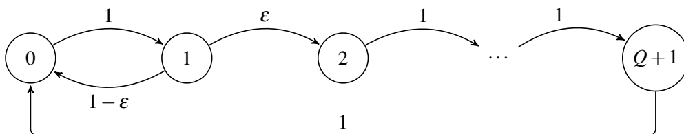
Figure 1: A simple example with Q + 2 states and only two possibilities for paths of T \wedge \tau .
