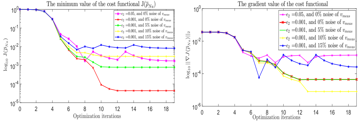
Fig. 2: Left: Log scale plot of the cost function \mathcal{I}(\bar{p}_{Na}) . Right: Log scale plot of the norm of its gradient during the optimization procedure.
