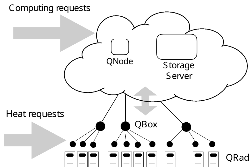
Figure 1: Scheme of the Qarnot platform.
