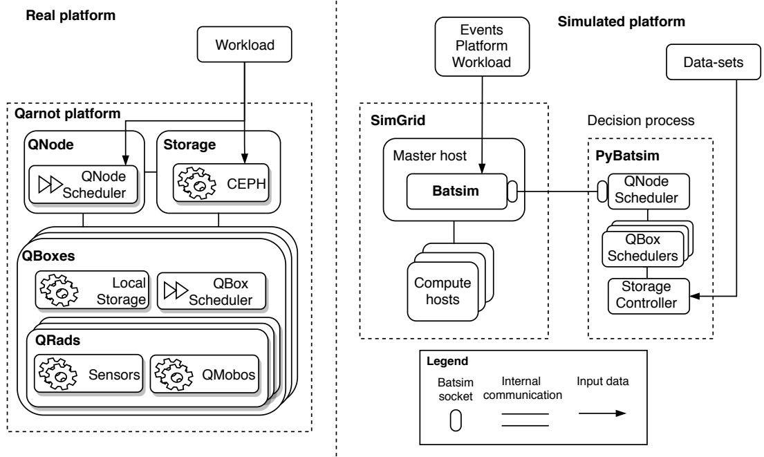
Figure 2: Comparison between the real and simulated Qarnot platform.
