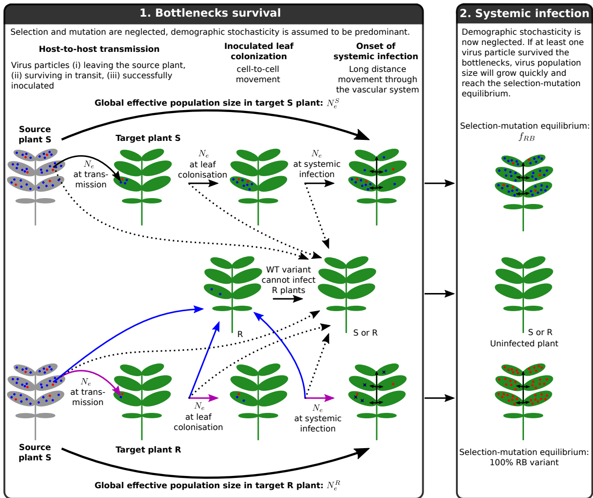
Figure S1: Modelling of the infection process. Wild-type (WT), resp. resistance-breaking (RB), virus variants are represented by blue, resp. red, dots. The source plant for infection is in grey and the target plant is in green. In the model, the infection of a new plant is decoupled into two steps: (1) bottleneck survival and (2) systemic infection. In the first step, only demographic stochasticity is considered. The effect of bottlenecks during host-to-host transmission, inoculated leaf colonization until the onset of systemic infection are summarised in the model in a global effective population size, which is N_e^S in susceptible (S) plants and N_e^R in resistant (R) plants (bold arrows). For the purpose of illustration, each bottleneck step is shown here, but the model only simulate a global, average, bottleneck. At each bottleneck step, survival of virus populations is represented by plain arrows whereas extinction is represented by dotted arrows. For a target S plant, plain black arrows indicate cases where either only the WT variant, only the RB variant or both variants pass through the bottleneck. For a target R plant, plain blue arrows indicate cases where only the WT variant passes through the bottleneck, whereas plain
