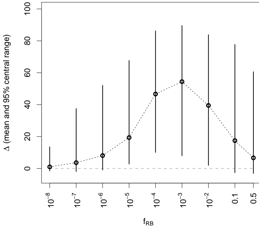
Figure 1: Additional relative benefit \Delta as a function of RB variant frequency in susceptible plants f_{RB} . All values of the other parameters are combined and \Delta corresponds to mean benefits over the 500 stochastic simulations for each combination of parameter values. Dots indicate means of \Delta and segments indicate 95% central range for each f_{RB} value (over all combinations of the other parameters). A grey dashed line indicates the limit \Delta = 0 .
