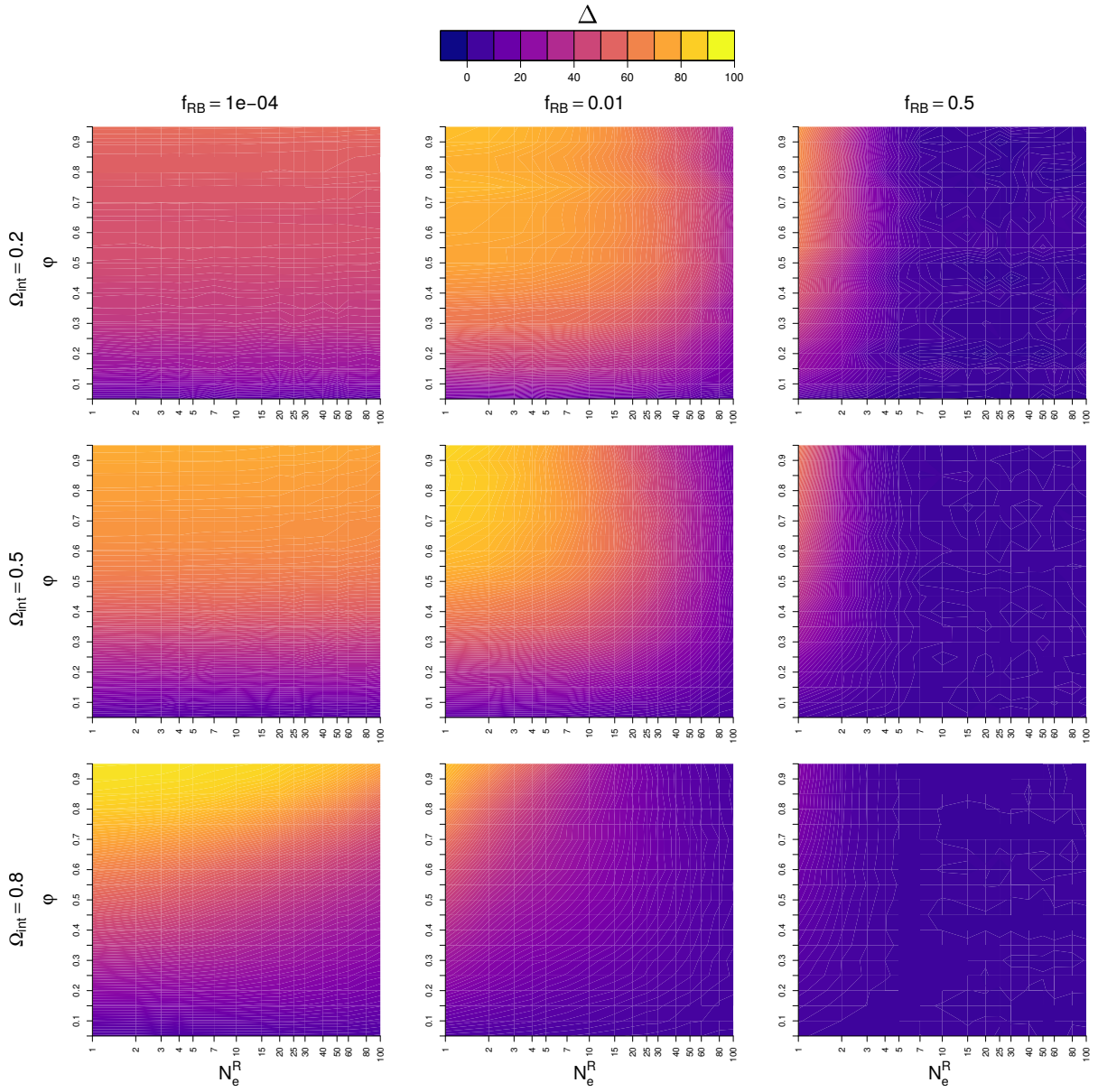
Figure 2: Effect of four parameters representative of the host, the virus, epidemic intensity and the field on the additional relative benefit \Delta . Contour plots representing \Delta as a function of the proportion of resistant plants \varphi (y-axis) and of virus effective population size in resistant plants N_e^R (x-axis). Panel lines represent contrasted epidemic intensities \Omega_{int} and panel columns contrasted RB variant frequencies in S plants f_{RB} .
