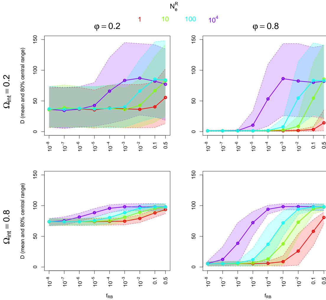
Figure S3: Relative damage D as a function of RB variant frequency in susceptible plants f_{RB} . Dots and plain lines are means, dashed lines and semi-transparent areas represent 80% central ranges. Colors represent various viral effective population sizes in R plants ( N_e^R = 10^4 : plants with monogenic resistance, N_e^R < 10^4 : plants with pyramided resistance). Panel lines represent distinct epidemic intensities \Omega_{int} and panel columns distinct proportions of resistant plants \varphi .
