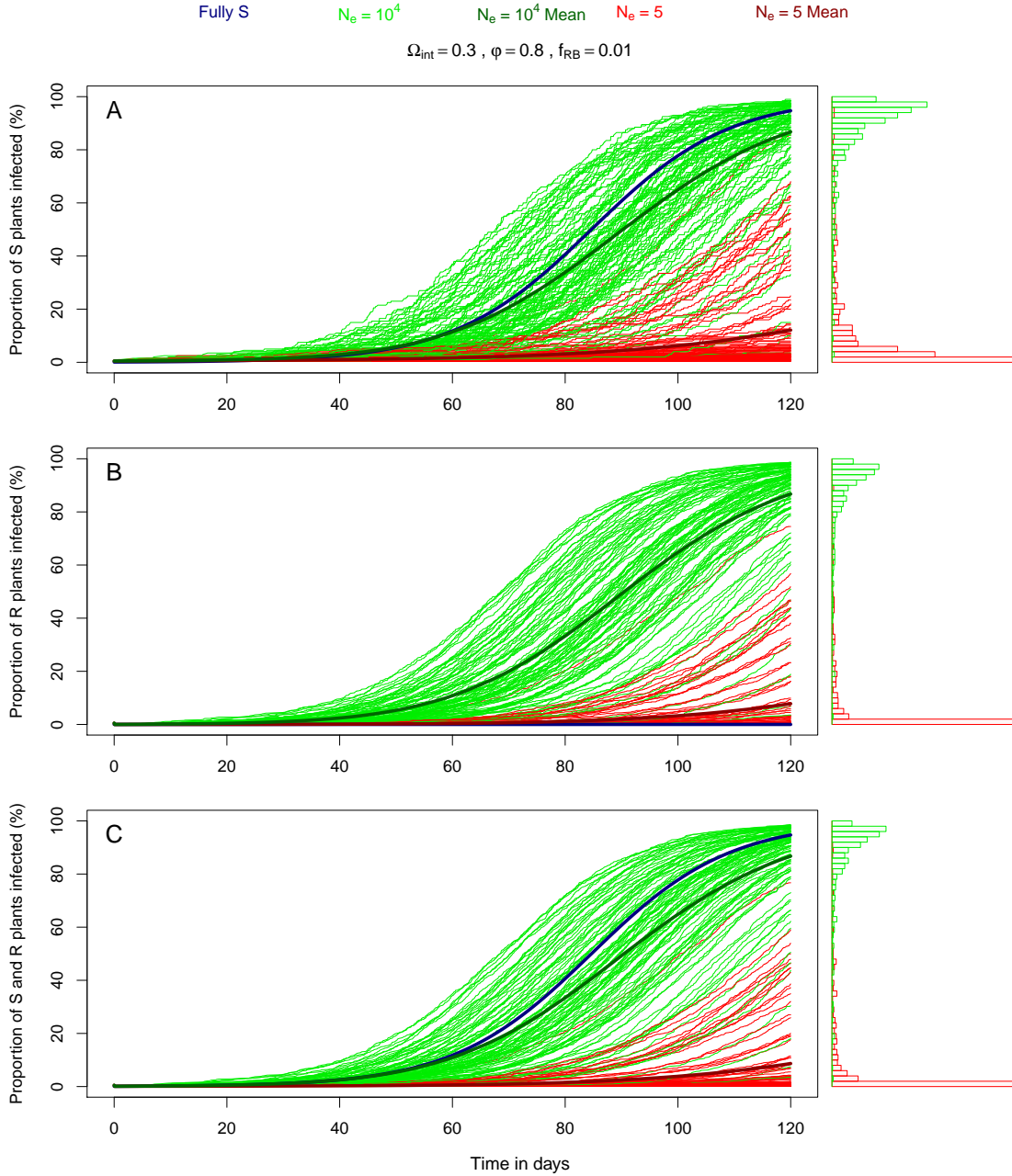
Figure S2: Epidemic dynamics. Evolution of the proportion of infected plants along the cropping season for susceptible S plants (A), resistant R plants (B) and both S and R plants (C). Blue thick curves are outputs in a fully S field (deterministic model) with reference epidemic intensity \Omega_{int} = 0.3 . Green and red curves are outputs for a proportion of R plants \varphi = 0.8 and a RB variant frequency in S plants f_{RB} = 0.01 (stochastic model). Green is for plants with monogenic resistance ( N_e^R = 10^4 ), red for plants with pyramided resistance ( N_e^R = 5 ). Thin curves are individual outputs, thick curves are corresponding means. The histograms represent the proportion of infected plants on the last day of the cropping season.
