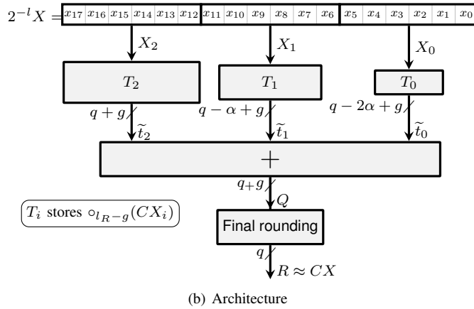
Fig. 6. FixRealKCM with an 18-bit input X split in 3 chunks of 6 bits.
