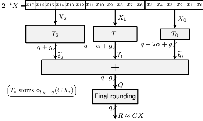
(b) Architecture
