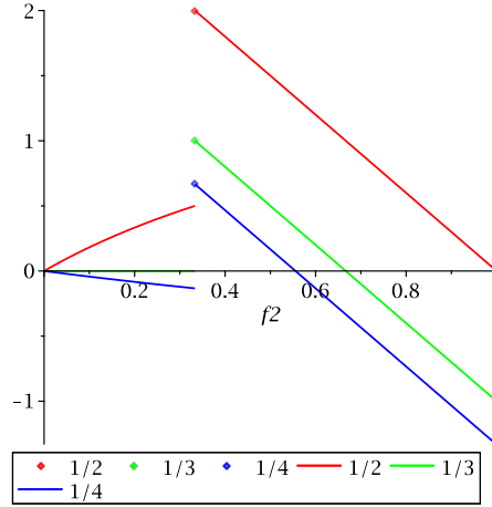
Figure 10: Gain of A as a function of f_2 for \beta_A = 1/2, 1/3, 1/4
