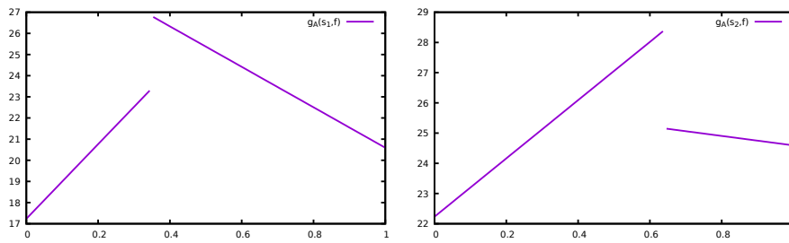
Figure 9: Value g_A(s, f) in Example 1, for s = s_1 (left) and s = s_2 (right)
