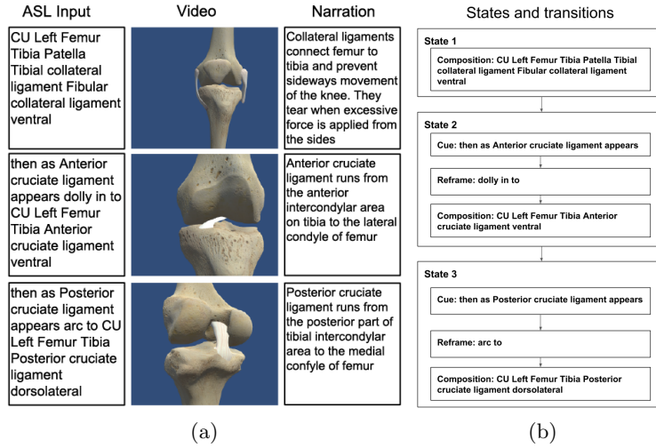
Fig. 1: Text-to-movie generation example with HFSM representation.
