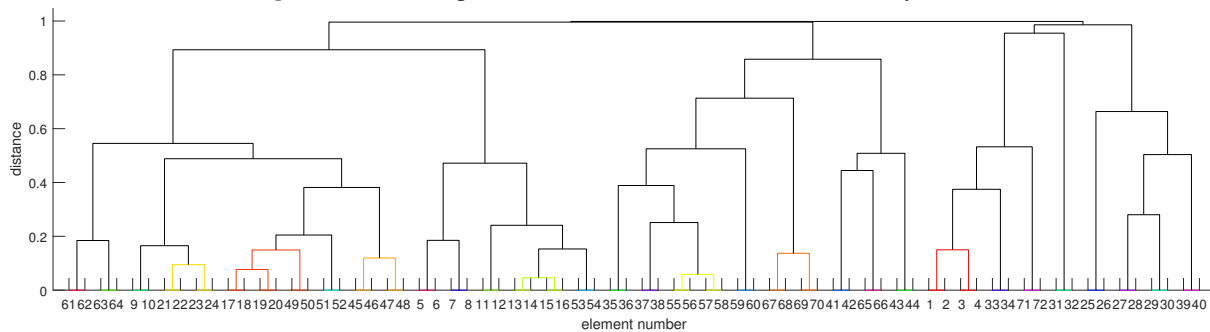
Figure 4: Dendrogram for clustering using 15 modes.
