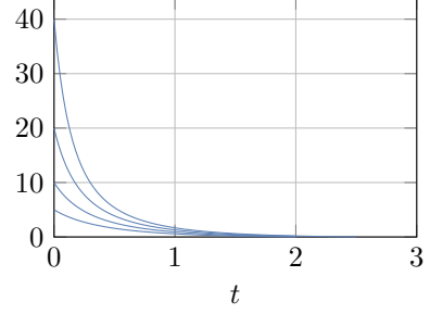
Figure 1: Solutions of system (7) for four different initial conditions.
