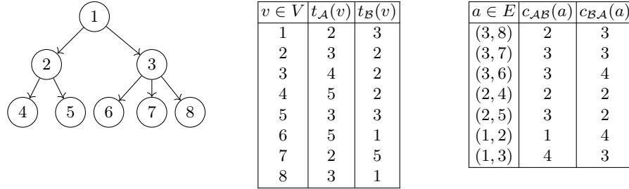
Fig. 2: An out-tree \mathcal{G} , duration of tasks and communication costs.
