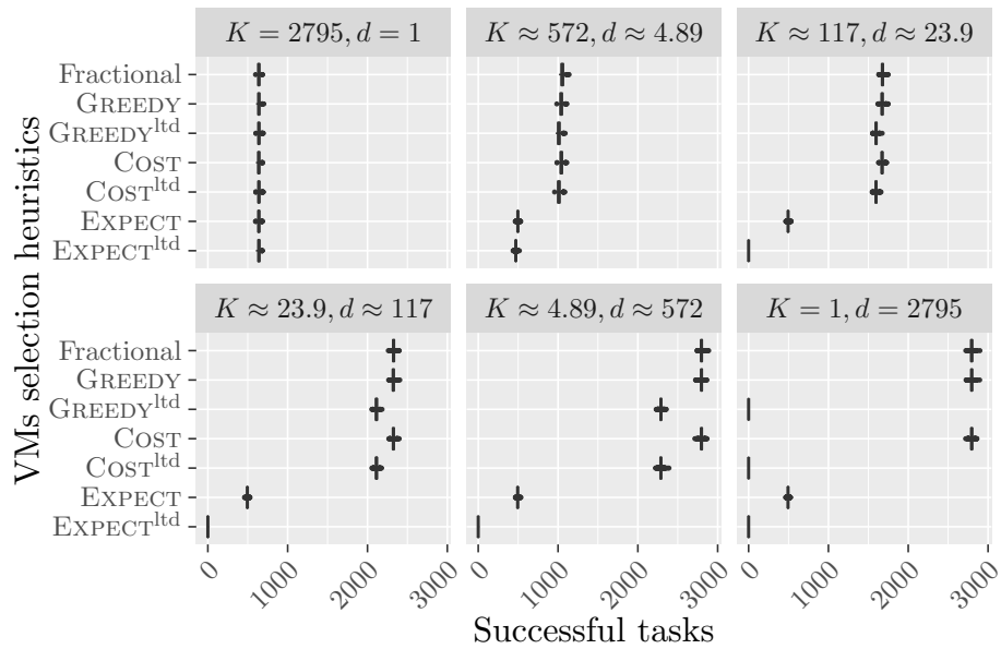
Figure 18: Number of successfully executed tasks of different methods to choose VMs when interrupting tasks with heuristic OPTRATIO . Platforms are generated with m_j = 10 , M = 60 , c_j = s_j^{1.5} and b \approx 2795 . The values for d and K follows a geometric progression between 1 and b \approx 2795 . Execution times follow an uniform distribution.
