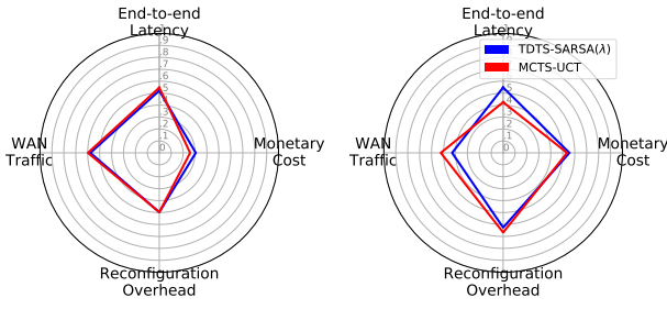
Figure 7: Cloud-only and TCEP with weights 0.7, 0.1, 0.1, and 0.1 for end-to-end latency, monetary cost, WAN traffic and reconfiguration overhead, respectively.
