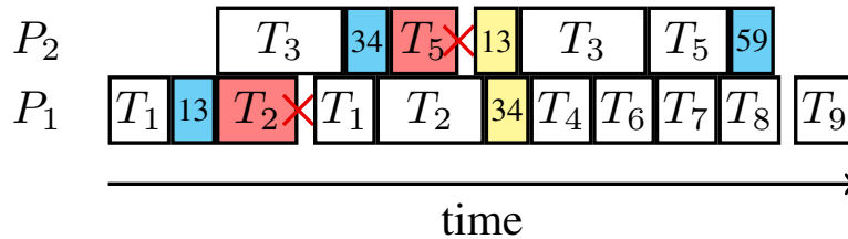
Figure 4. Sample execution of the application in Figure 3 with two failures striking during the execution of T_2 on P_1 and that of T_5 on P_2 , with crossover checkpoints. Label ij indicates the file from T_i to T_j . Now T_4 can start before the re-execution of T_3 since its output was checkpointed.
