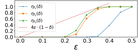
Figure 2: Values of \eta_{f_i,\varepsilon}(\delta) for \delta = 0.3
