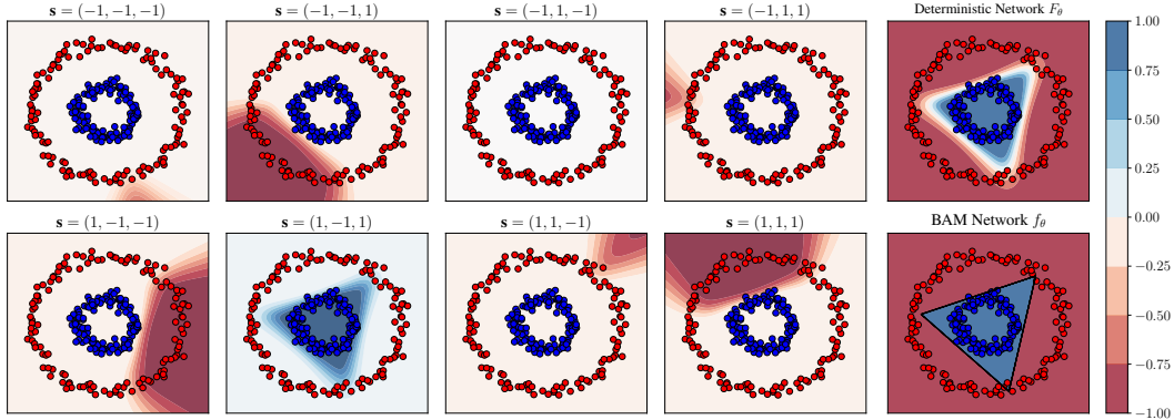
Figure 3: Illustration of the proposed method in Section 3 for a one hidden layer network of size d_1 = 3 , interpreted as a majority vote over 8 binary representations \mathbf{s} \in \{-1, 1\}^3 . For each \mathbf{s} , a plot shows the values of F_{w_2}(\mathbf{s})\Psi_{\mathbf{s}}(\mathbf{x}, \mathbf{W}_1) . The sum of these values gives the deterministic network output F_{\theta}(\mathbf{x}) (see Equation 9). We also show the BAM network output f_{\theta}(\mathbf{x}) for the same parameters \theta (see Equation 6).
