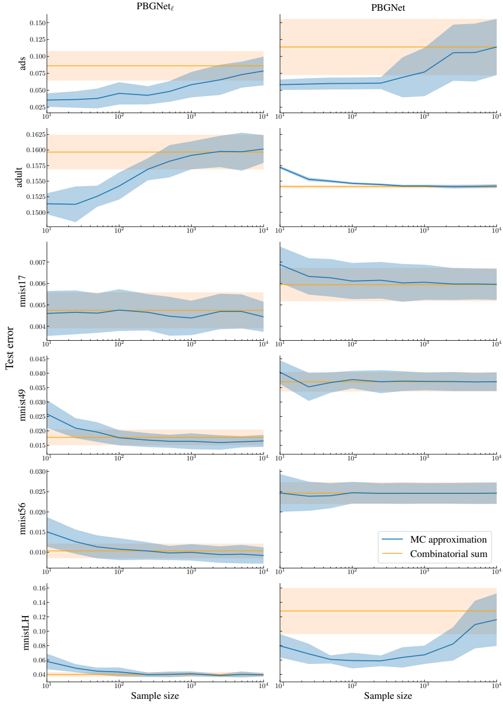
Figure 5: Impact of the sample size T on stochastic gradient descent solution test error for \text{PBGNet}_\ell and \text{PBGNet} . Network parameters were fixed with a single hidden layer of size 10 and trained with initial learning rate of 0.1. For each sample size values and the combinatorial sum approach, 20 repetitions of the learning procedure with different random seeds were performed. The test error mean of the learned models is displayed by the bold line, with standard deviation shown with the shaded areas.
