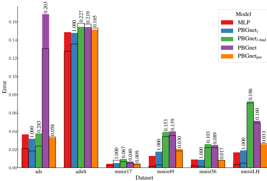
Figure 4: Visualization of experiments results for the models on the binary classification datasets. The colored bars display the test error while the black outlined bars exhibit the train error. The PAC-Bayesian generalization bounds are identified on the top of the bars and hold with probability 0.95.
