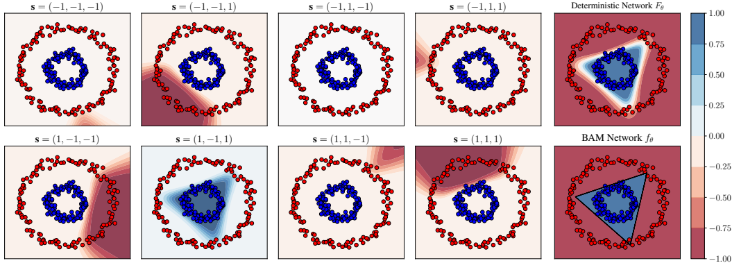
Figure 3: Illustration of the proposed method in Section 3 for a one hidden layer network of size d_1 = 3 , interpreted as a majority vote over 8 binary representations \mathbf{s} \in \{-1, 1\}^3 . For each \mathbf{s} , a plot shows the values of F_{w_2}(\mathbf{s})\Psi_{\mathbf{s}}(\mathbf{x}, \mathbf{W}_1) . The sum of these values gives the deterministic network output F_{\theta}(\mathbf{x}) (see Equation 9). We also show the BAM network output f_{\theta}(\mathbf{x}) for the same parameters \theta (see Equation 6).
