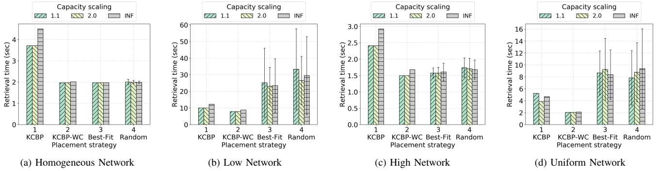
Fig. 2. Retrieval time for Synthetic networks.
