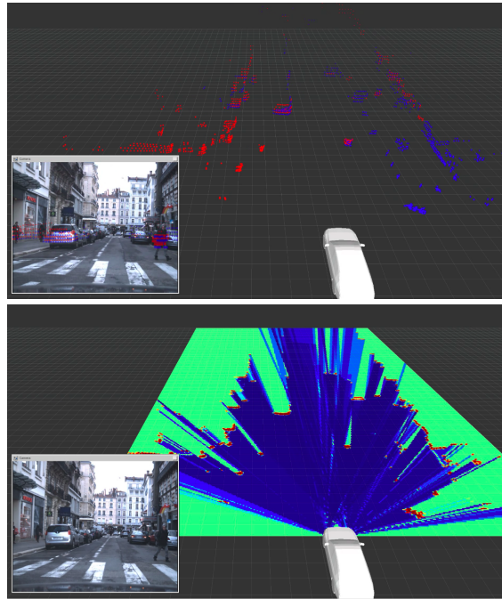
Fig. 3. Data fusion in an occupancy grid. Data from each of the 2 lidars are used to generate occupancy grids using sensor models, which are then combined by using Bayesian fusion.
