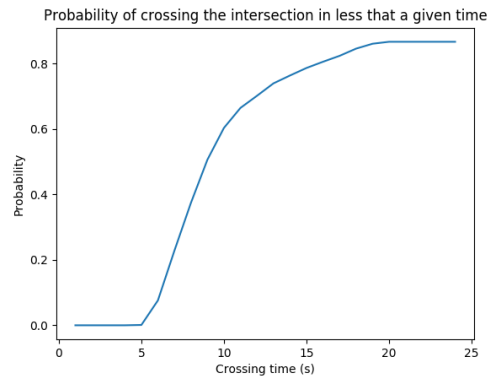
Fig. 12. Probability of crossing the intersection in less than a given time.
