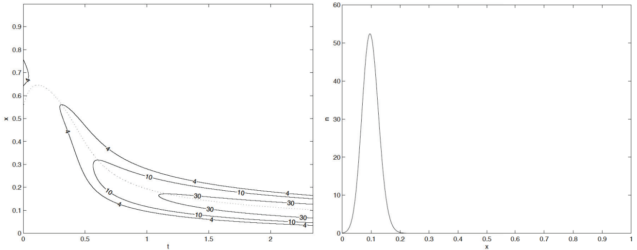
Figure 5: Healthy (or sensitive) cell population case . Left panel: starting from an arbitrary median phenotype x=0.5 , level sets of a drug-sensitive population in the (t,x) plane (time in abscissae and phenotype in ordinates). Right panel: asymptotic distribution of this population according to the drug resistance phenotype x \in [0,1] . [Sensitive (or healthy) cell population case: again, illustration of Gause's exclusion principle] here with \theta_H=0 (no mutations) and \mu_H=0 (no drug-induced resistance), with u(t) = Cst [29]
