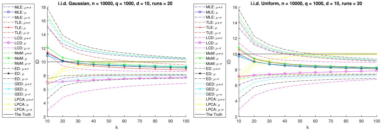
Figure 3: Means and standard deviations of estimated ID values, for dimensionality 10 and various neighborhood sizes. Left: i.i.d. Gaussian data. Right: i.i.d. uniform data.
