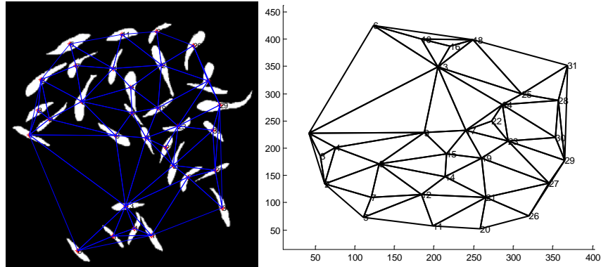
Fig. 6. Delaunay Triangulation
