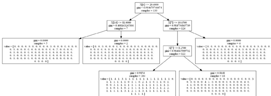
Fig. 3 The 3 Layers Decision Tree Generated by CART Algorithm Processing the Rice
