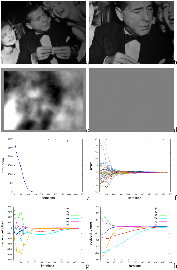
Figure 10. Experiment with real planar scene (a) initial image acquired by the camera \mathbf{I}(\mathbf{r}) , (b) image \mathbf{I}^* acquired from the desired position, (c,d) error [\mathbf{U}\mathbf{w}(\mathbf{r})]_{50} - [\mathbf{U}\mathbf{w}^*]_{50} between reconstructed image for initial and desired position (a,b,c,d) are used for visualization but are not used in the algorithm. Only the error \mathbf{w}(\mathbf{r}) - \mathbf{w}^* plotted in (f) is considered, (e) \|\mathbf{w}(\mathbf{r}) - \mathbf{w}^*\| (g) camera velocity (in m/s and rad/s) (h) positioning error (in m and rad).
