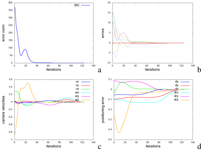
Figure 6. Experiment \text{exp-w6} : Positioning task using compact eigenspace representation with K = 6 (a) error norm \| \mathbf{w}(\mathbf{r}) - \mathbf{w}^* \| (b) errors w_i(\mathbf{r}) - w_i^* , i = 1..6 (c) camera velocity (in m/s and rad/s) (d) positioning error (in m and rad)
