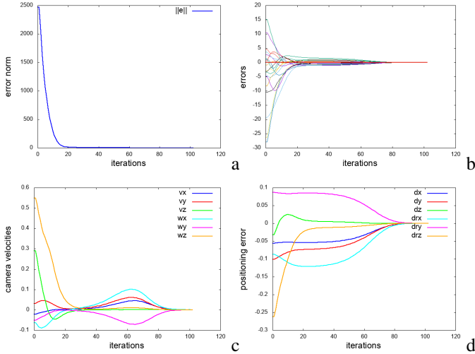
Figure 7. Experiment \text{exp-w20} : Positioning task using compact eigenspace representation with K = 20 (a) error norm \| \mathbf{w}(\mathbf{r}) - \mathbf{w}^* \| (b) errors w_i(\mathbf{r}) - w_i^* , i = 1..20 (c) camera velocity (in m/s and rad/s) (d) positioning error (in m and rad).
