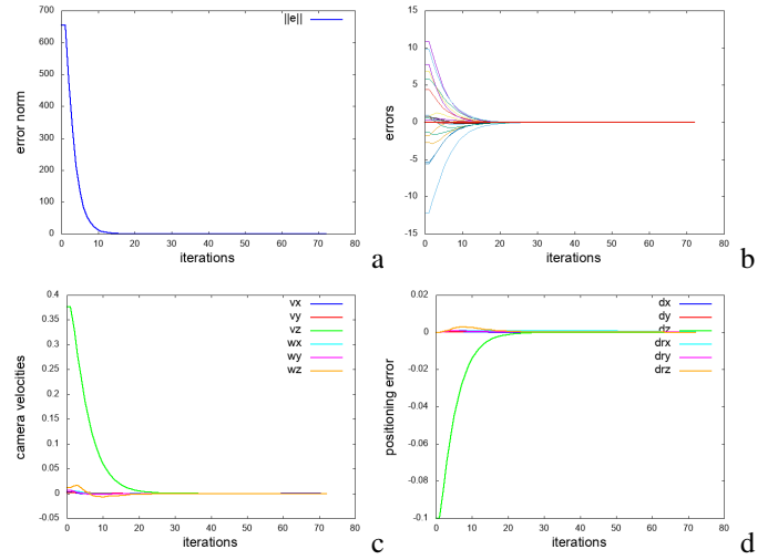
Figure 8. Positioning task using compact eigenspace representation with K = 20 for a pure translation motion \Delta \mathbf{r} = (0, 0, 0.1m, 0, 0, 0) (a) error norm \| \mathbf{w}(\mathbf{r}) - \mathbf{w}^* \| (b) errors w_i(\mathbf{r}) - w_i^* , i = 1..20 (c) camera velocity (in m/s and rad/s) (d) positioning error (in m and rad)
