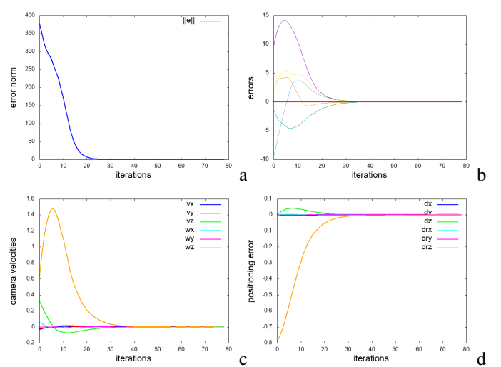
Figure 9. Positioning task using compact eigenspace representation with K = 6 for a pure rotation motion around Z axis. \Delta \mathbf{r} = (0, 0, 0, 0, 0, 45^\circ) (a) error norm \| \mathbf{w}(\mathbf{r}) - \mathbf{w}^* \| (b) errors w_i(\mathbf{r}) - w_i^* , i = 1..20 (c) camera velocity (in m/s and rad/s) (d) positioning error (in m and rad)
