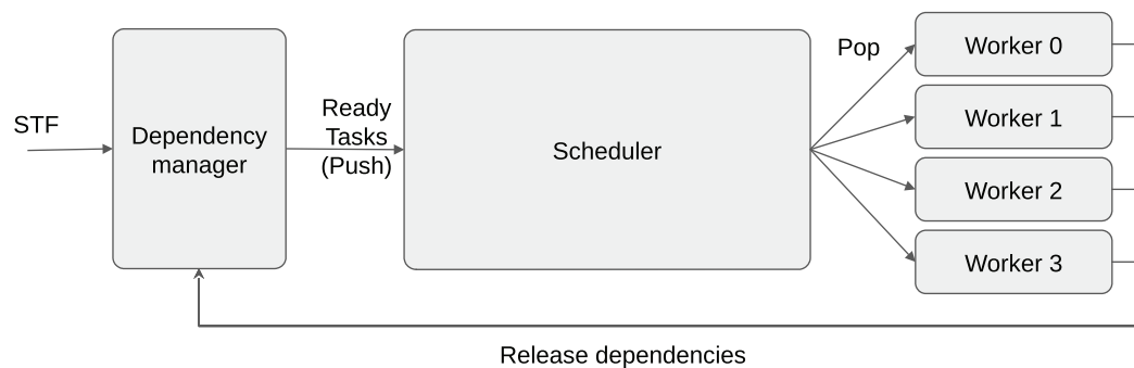
Figure 1 Schematic view of task-based runtime system organization. A program can be described using the sequential task flow (STF) model and converted into tasks/dependencies by the RS. When dependencies are released, the newly ready tasks are pushed into the scheduler. When a worker is idle, it calls the pop function of the scheduler to request a task to execute.
