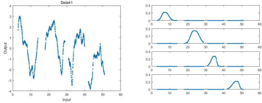
Fig. 4. The dataset with the least degree of overlap from MGP with 4 components. Fig. 5. The distribution of the probability density function of the input on each Gaussian processes component.
