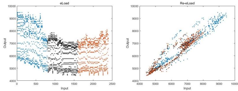
Fig. 1. The sketch of the eLoad data. Fig. 2. The sketch of the transformed eLoad data.
