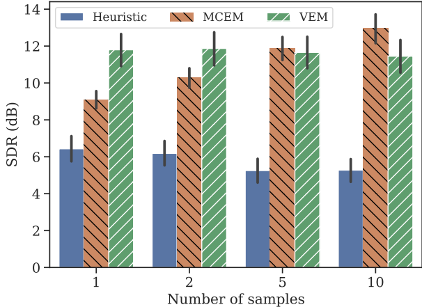
Figure 1: SDR as a function of number of samples M for an input SNR of 0dB. using MH for reconstruction. Heuristic, MCEM and VEM methods are defined in Section 4.1. Errors bars indicate 95% confidence interval.
