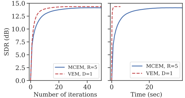
Figure 2: Average convergence speed. SDR as a function of (left) number of iteration and (right) absolute time.
