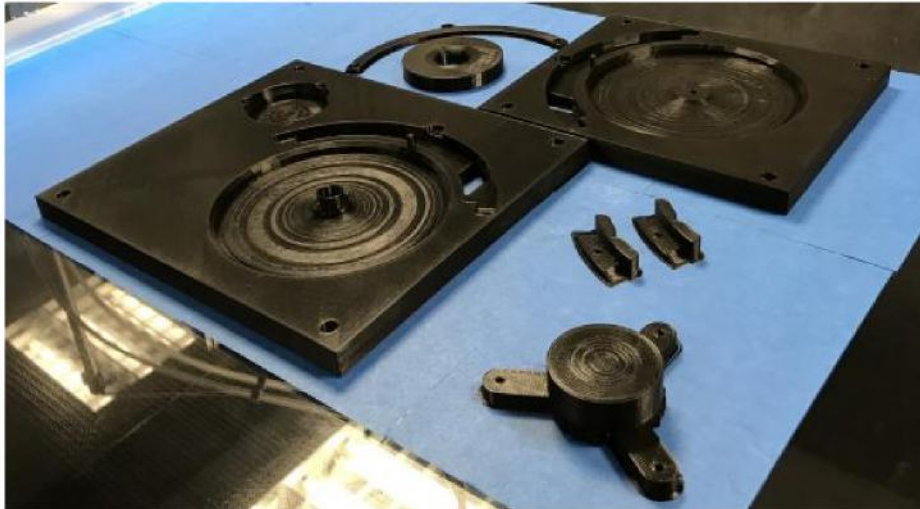
Fig. 8. An example of 3D printed parts used as fixture nests in a TQC machine
