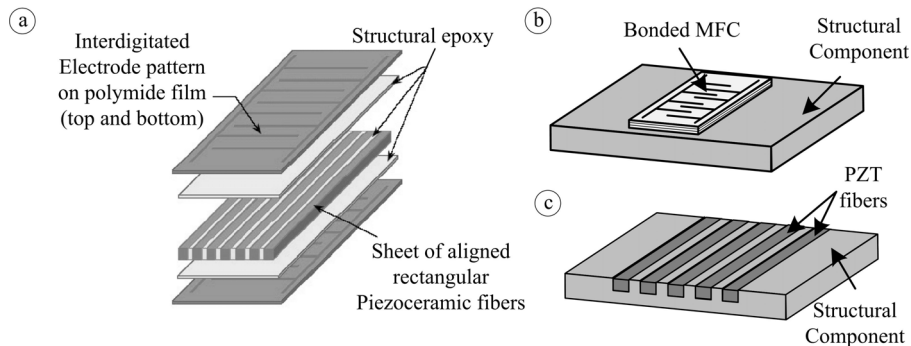
Fig. 1 a) Design of Macro Fiber Composites (MFC) [1]; b) Application of MFC with adhesive on the surface of a structural component; c) New approach with structural integration of PZT fibers into a structural component
