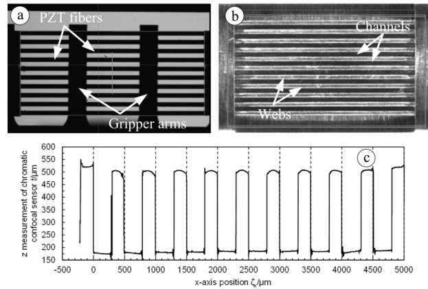
Fig. 7. a) Machine vision image for a PZT fiber array with transmitted coaxial light; b) Machine vision image for microstructure with side lighting; c) Measuring result for the chromatic confocal sensor
