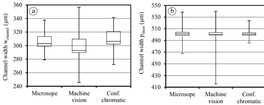
Fig. 10. a) Box plot for Channel width; b) Box plot for the pitch in the microstructured sheet metal
