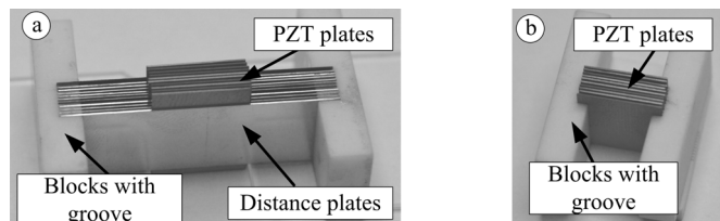
Fig. 8. a) Stacking device 1 with distance plates; b) Stacking device 2
