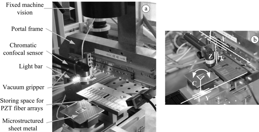
Fig. 5. a) Basic structure of the micro assembly system; b) Assignment of the axes
