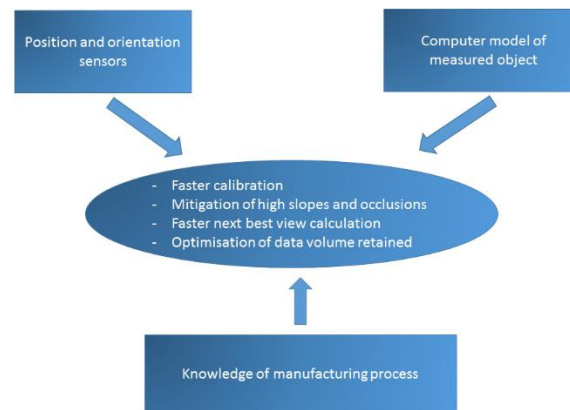
Fig. 4. A priori data used for the fringe projection system under development at Nottingham.
