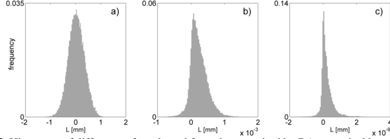
Fig. 3. Histogram of differences L evaluated from data acquired by RA on optical breadboard plate: a) based on original, uncorrected locations of fiducials; b) based on fiducials after the first step of RBC restoration; c) based on fiducials after the second, final step of RBC restoration.
