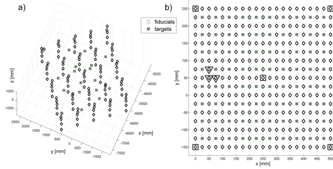
Fig. 1. a) 3D data: locations of 125 fiducials and 16 targets plotted in coordinate frame of LT. b) 2D data: locations of 277 fiducials and 80 targets displayed in world coordinate frame. Large squares mark locations of five fiducials used to perform the registration of original, uncorrected data. Triangles mark locations of three fiducials used to perform the registration after RBC was restored in the set of fiducials.
