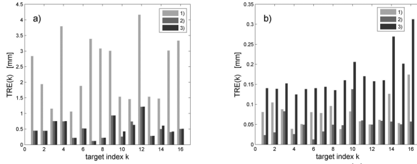
Fig. 4. Target registration error calculated using three methods: 1) TRE_u(k) for uncorrected, average fiducials and targets; 2) TRE_c(k) for corrected, average fiducials and targets; 3) corrected, instantaneous fiducials and targets – displayed is median of N = 200 instantaneous errors TRE_c^{(n)}(k) : a) data acquired by System A and LT; b) data acquired by System B and LT.
