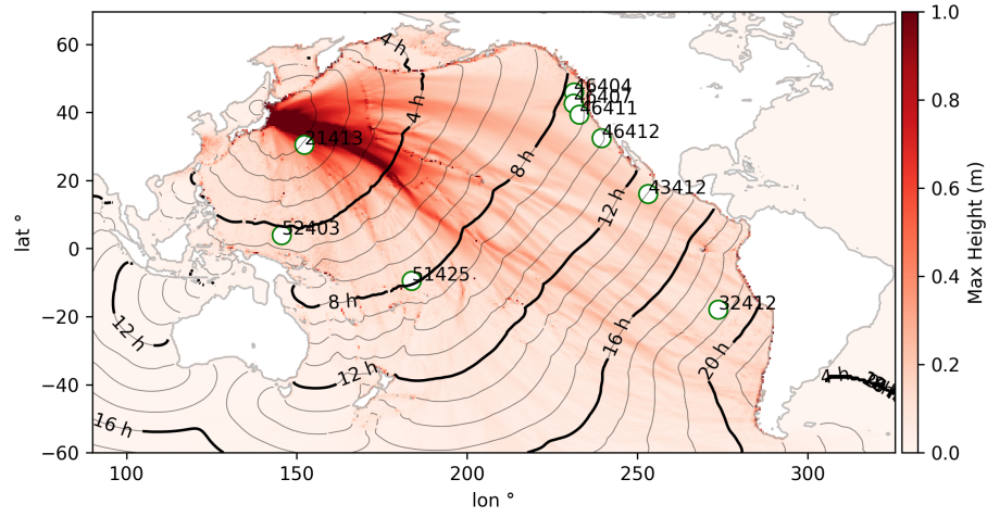
Figure 8: “Heat maps” of maximum wave amplitude and arrival time isochrones calculated by Nami for the 9.1 Mw scenario of Tohoku, Japan, 2011 and DART buoys locations.
