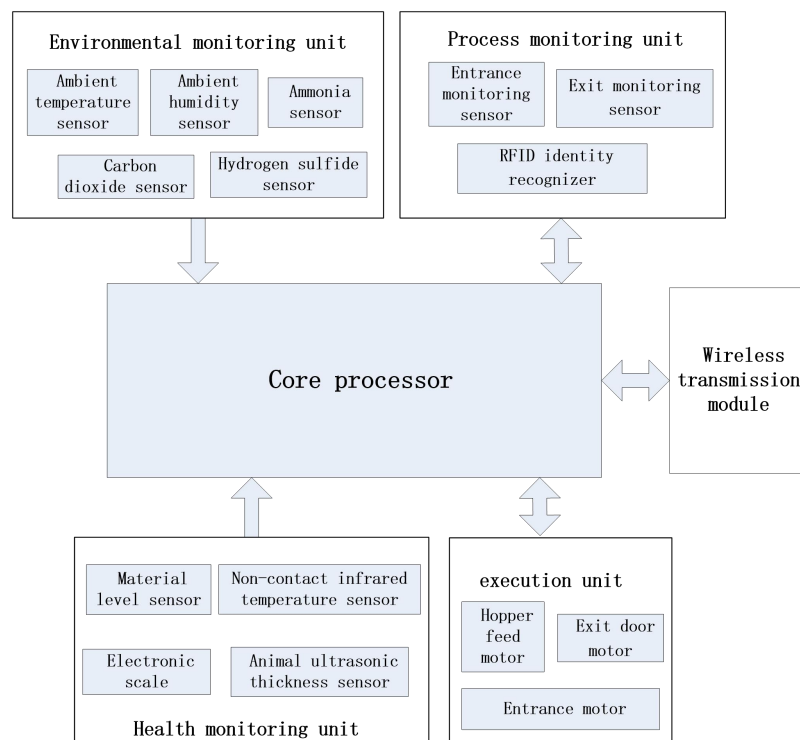
Fig.2 The hardware of pig intelligent feeding equipment
