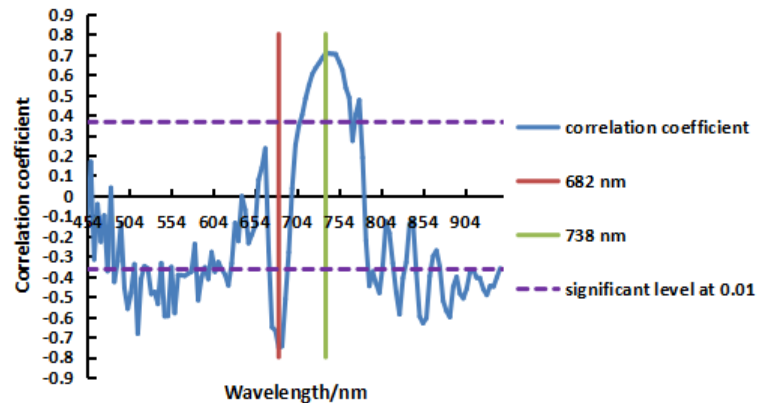
Fig.8 Correlation between first derivative of spectrum and nitrogen content in leaves at grain filling stage
