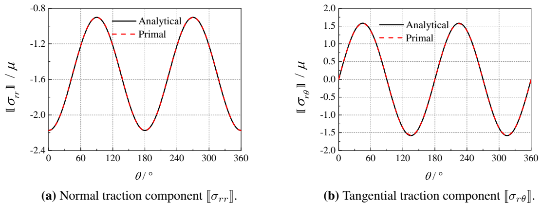
Figure 15: Traction jumps across the interface for the inextensible shell type interphase model.
