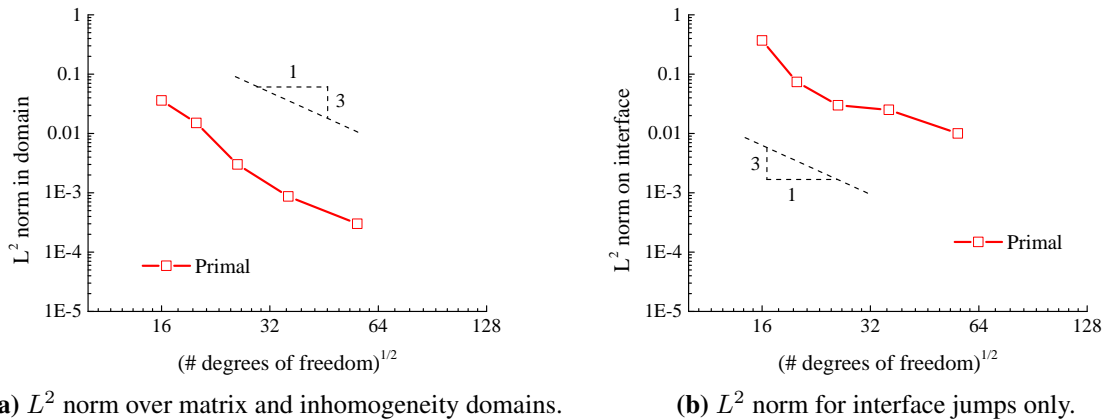
Figure 20: Convergence of the stress in the L^2 -norm for cubic elements.
