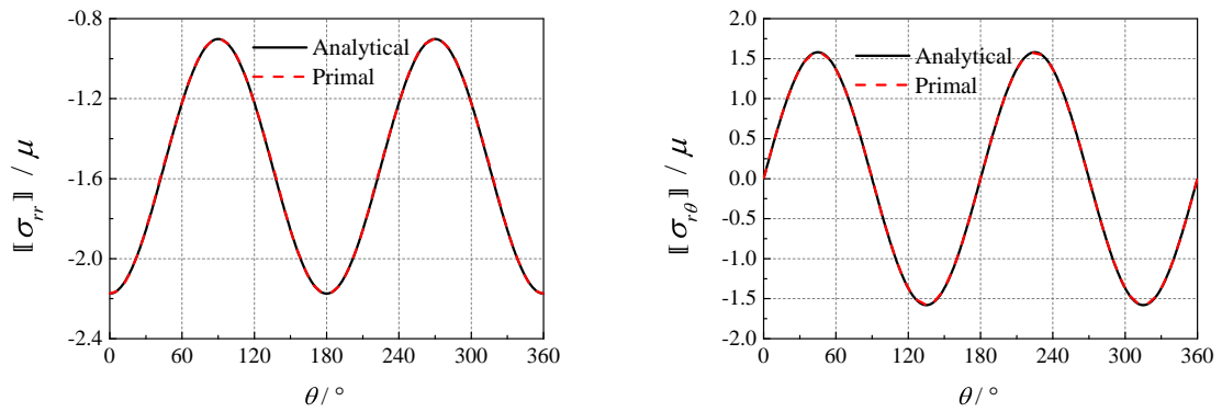
(a) Normal traction component [[\sigma_{rr}]] .
