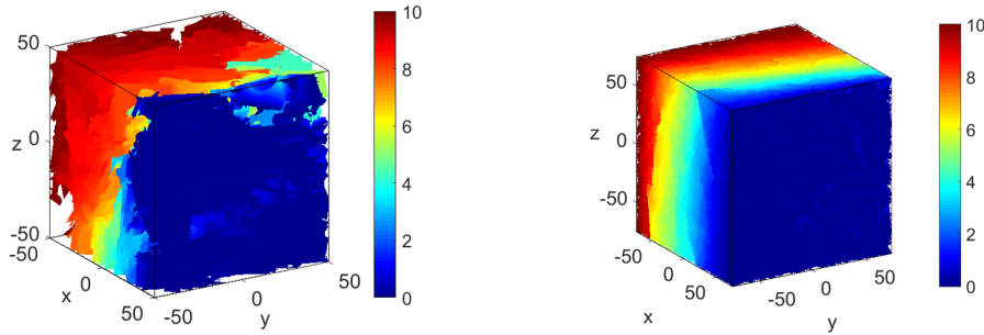
Figure 4: Mean hydraulic heads computed for permeameter boundary conditions in the x direction. Left, DFN100 (fine) test case. Right, DFN150 test case.
