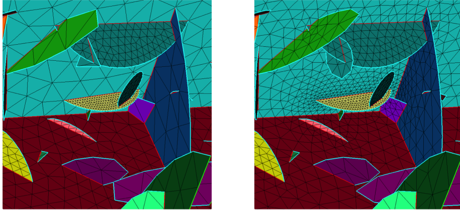
Figure 3: Nonconforming and conforming meshes.
