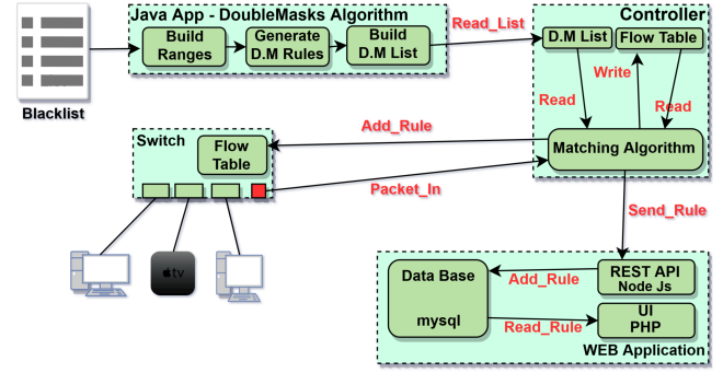
Fig. 10: Architecture and set-up of our SDN network.
