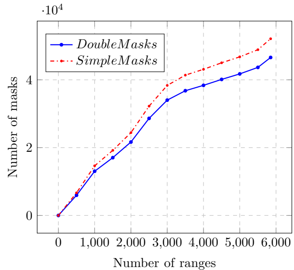
Fig. 6: Number of masks computed respectively by DoubleMasks and SimpleMasks algorithms using the IP blacklist dataset.
